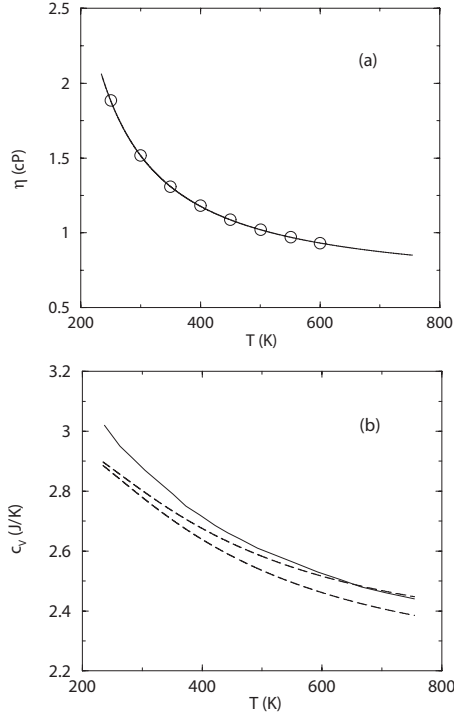
FIG. 1. (a) Circles are experimental data of viscosity of mercury, line is the fit and extrapolation using the Vogel-Fulcher-Tammann formula; (b) solid line is the experimental c_v for mercury. Dashed lines are calculated values, using \tau_{mt}G_\infty of 0.55 \times 10^{-3} Pa s (top) and 0.57 \times 10^{-3} Pa s (bottom).
